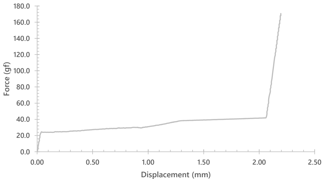
Kailh Low Profile Saker (Upstroke)
